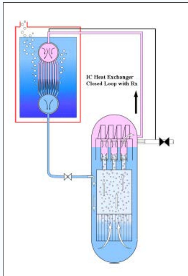
Figure 21. Isolation Condenser System
